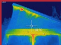
Recording at -20 °C with BlidimaX® and BlidimaX® roof
